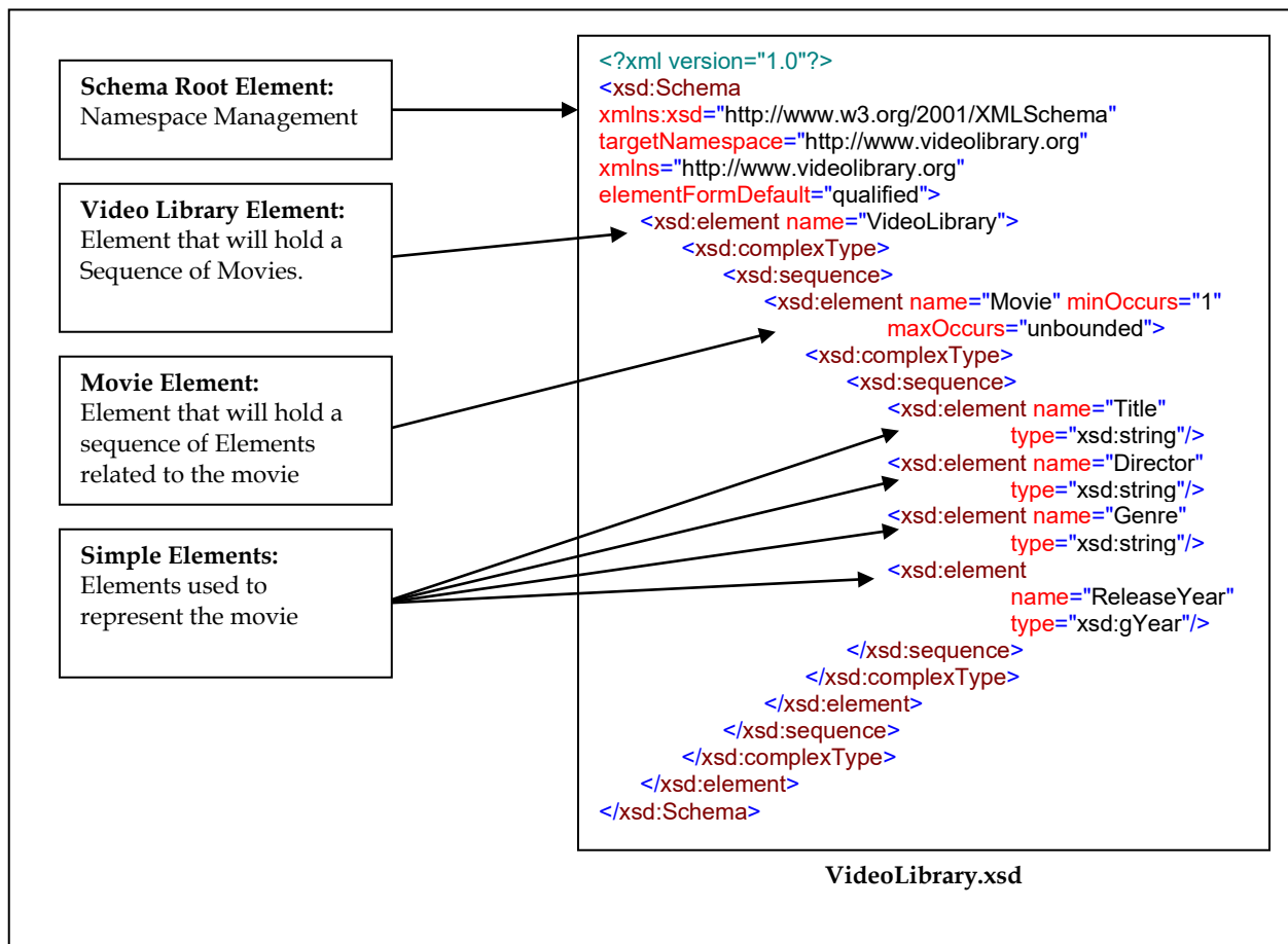
Figure 2.1 – Basic XML Schema Example
