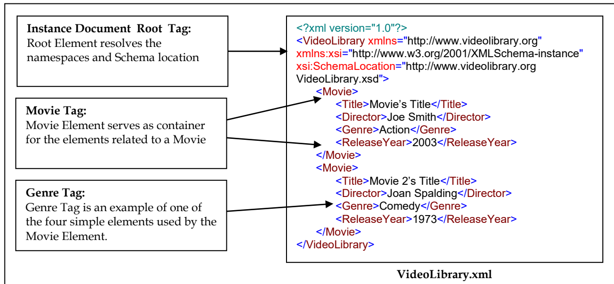
Figure 2.2 - Basic XML Instance Document Example
