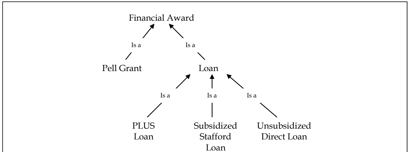
Figure 3.1 - Design by Subclassing Diagram
