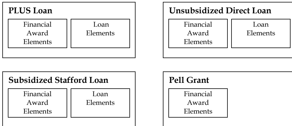
Figure 3.2 - Design by Composition Diagram
